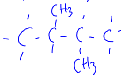
2,3-dimethylbutane
