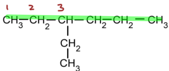
ethylhexane
