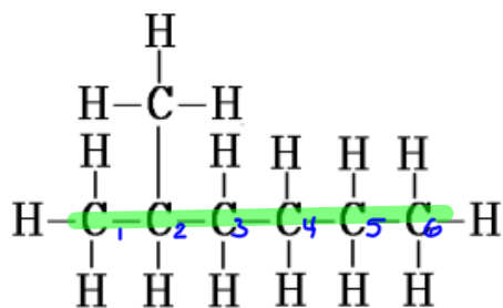
2-methylhexane
