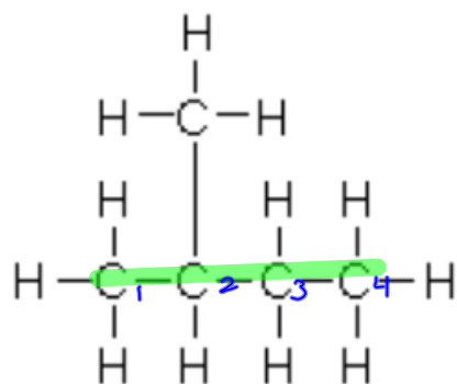
methylbutane
