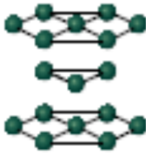
Hexagonal close-packed
