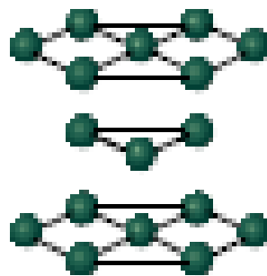
Hexagonal close-packed
