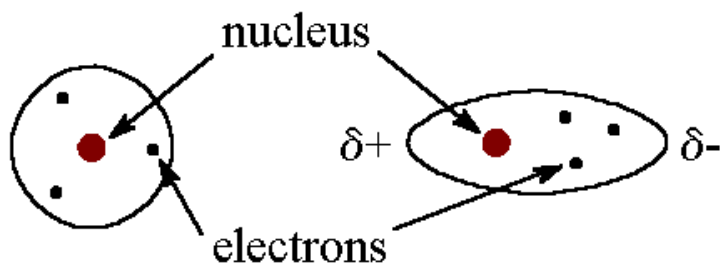
symmetrical distribution
