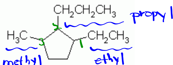
1-ethyl-3-methyl-2-propylcyclopentane
